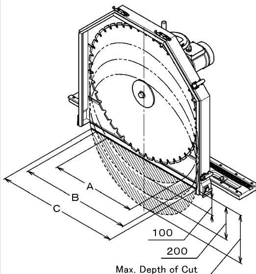
The relationship between the diameter of Blade and Max. Depth and Width of Cut
